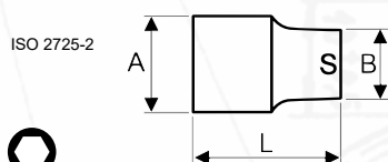
ISO 2725-2 1/2" Hlavice průmyslová Drive CrMo + trn, o-kroužek 1/2" Impact socket Drive CrMo + pin, o-ring 1/2" Schlag-Steckschlüssel Drive CrMo + Dorn, O-Ring
