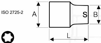
ISO 2725-2 1/2" Hlavice průmyslová TORX CrMo + trn, o-kroužek 1/2" Impact socket TORX CrMo + pin, o-ring 1/2" Industrieinsatz TRX CrMo + Dorn, O-Ring
