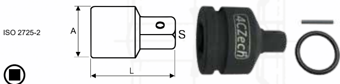
ISO 2725-2 3/4" - 1/2" Redukce průmyslová CrMo + trn, o-kroužek 3/4" - 1/2" Impact coupler CrMo + pin, o-ring 3/4" - 1/2" Schlag-Reduction + Dorn, O-Ring
